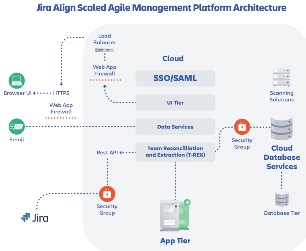
Figure 1: Jira Align Infrastructure
